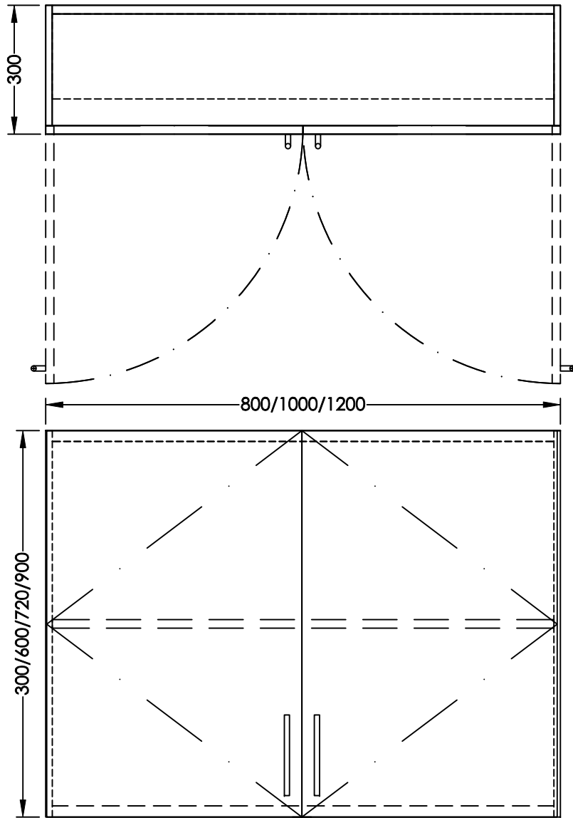
FRONT ELEVATION
